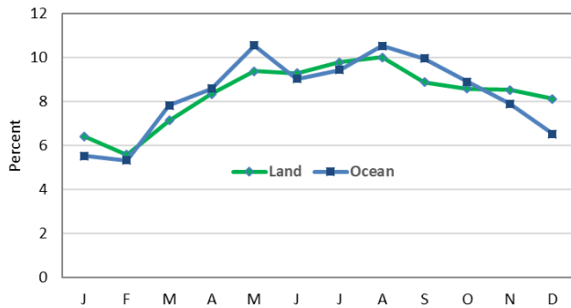
Fig. 4. Lightning stroke percentages by month over all land and ocean areas of the world.
