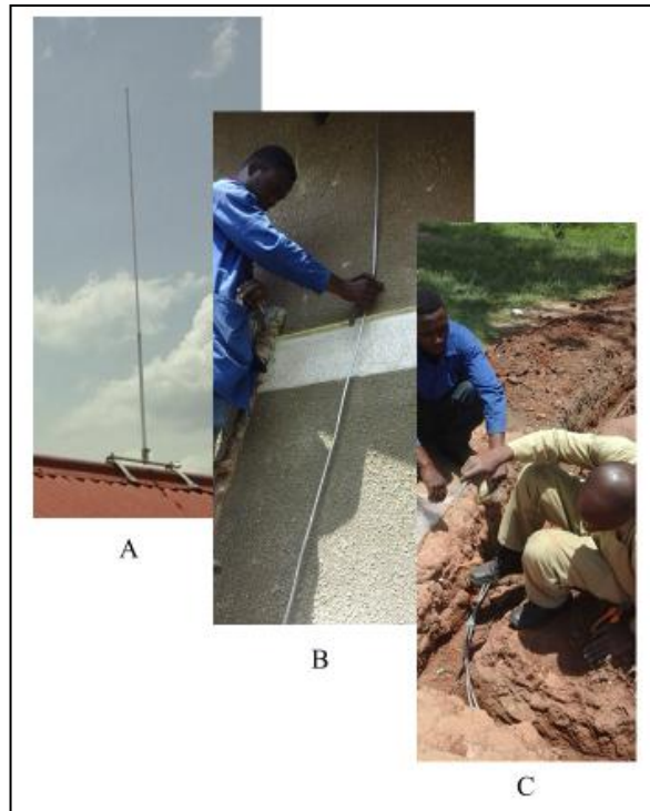
Fig. 17.1 Installation of A: Air terminal, B: Down conductor, and C: Ground terminal at school in Uganda (courtesy ACLENet)
