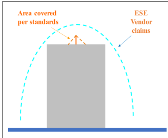
Fig. 17.4 ESE manufacturers claimed that by having a higher effective height, a larger radius of coverage was achieved, necessitating fewer rods to cover the area to be protected. This was proven to be a false claim in independent scientific trials (courtesy C. Gomes)
