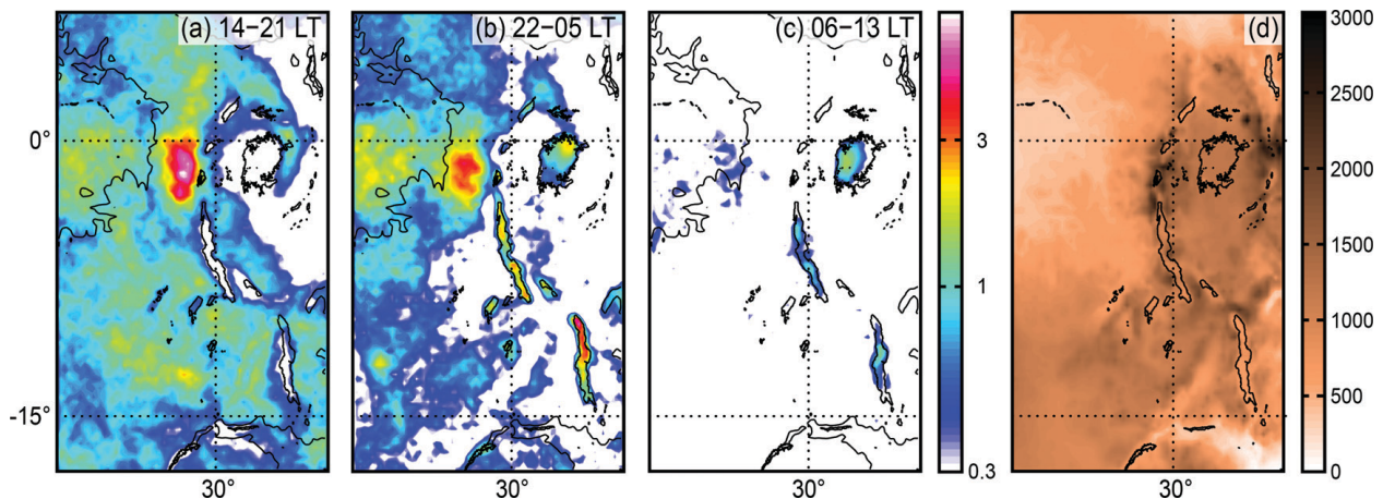
FIG. 8. As in Fig. 7, but for tropical Africa for all months. Local time given for Kampala, Uganda.
