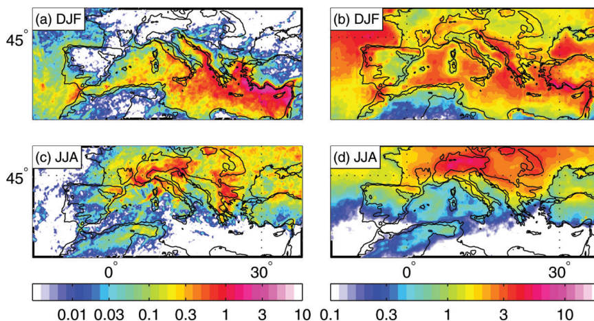
FIG. 5. (a),(c) WLLN lightning stroke frequency ( \text{km}^{-2} \text{yr}^{-1} ) and (b),(d) TRMM 3B42 precipitation ( \text{mm day}^{-1} ; both at 0.25^\circ \times 0.25^\circ resolution) during (a),(b) DJF and (c),(d) JJA. Black contours indicate the 500-m elevation.
