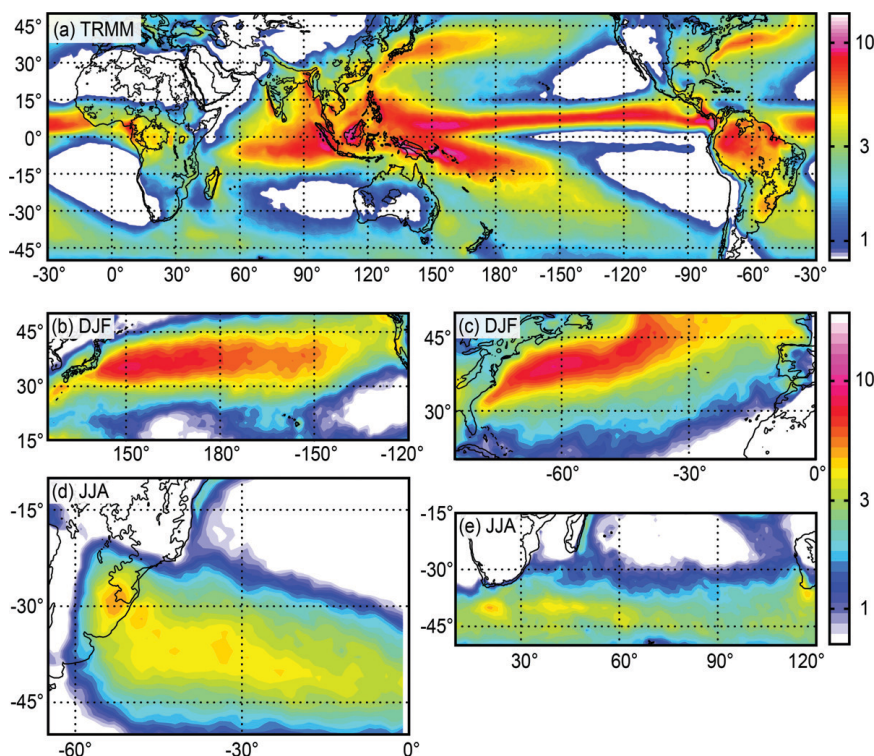
FIG. 3. TRMM (a) annual-mean and (b)–(e) seasonal-mean precipitation ( \text{mm day}^{-1} ; 1^\circ \times 1^\circ resolution). Black contours indicate the 500-m elevation.
