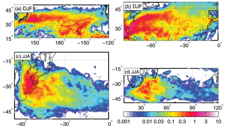
FIG. 4. WWLLN seasonal-mean lightning stroke frequency ( \text{km}^{-2} \text{yr}^{-1} ; 1^\circ \times 1^\circ resolution) during (a),(b) Dec–Feb (DJF) and (c),(d) Jun–Aug (JJA). Black contours indicate the 500-m elevation.
