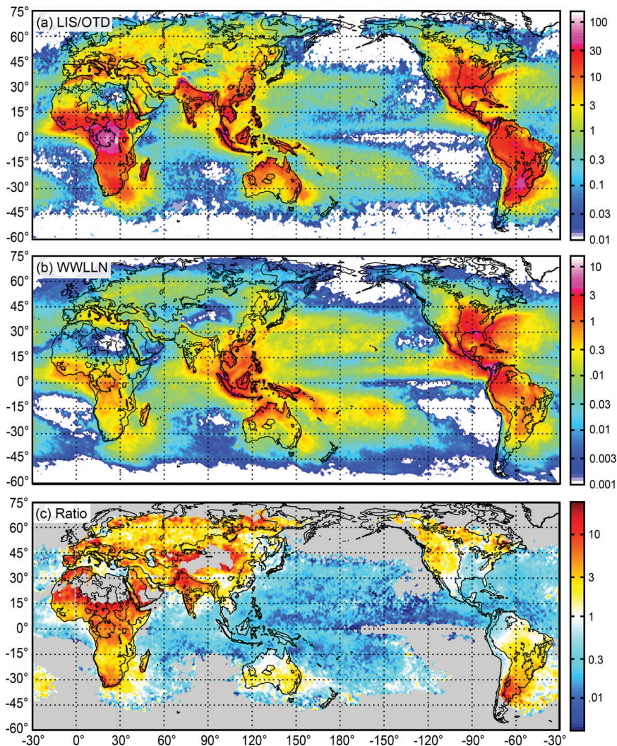
FIG. 2. Annual-mean frequency of occurrence of lightning from (a) LIS/OTD (flashes \text{km}^{-2} \text{yr}^{-1} ) and (b) WWLLN (strokes \text{km}^{-2} \text{yr}^{-1} ). (c) Ratio of LIS/OTD flashes to WWLLN strokes, scaled by the mean of each dataset (gray shading indicates either no LIS/OTD lightning flashes or WWLLN lightning stroke frequency < 0.01 \text{ km}^{-2} \text{yr}^{-1} ; see text for details). All fields have been averaged on a 1^\circ \times 1^\circ grid. Black contours indicate the 500-m elevation.
