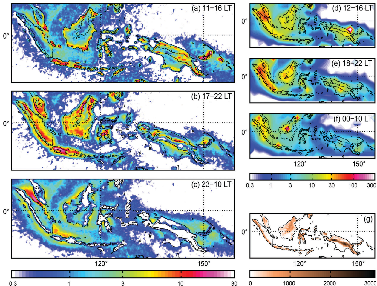
FIG. 6. (a)–(c) WWLLN lightning stroke frequency ( \text{km}^{-2} \text{yr}^{-1} ; hourly, 0.25^\circ \times 0.25^\circ resolution) and (d)–(f) LIS/OTD lightning flash frequency ( \text{km}^{-2} \text{yr}^{-1} ; two hourly, 2.5^\circ \times 2.5^\circ resolution) for indicated time intervals during all months. Local time given for Singapore. Black contours indicate the 500-m elevation. (g) Elevation (m).
